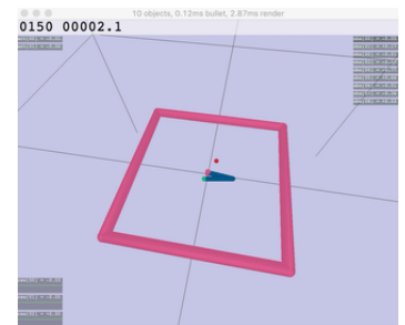
(l) SLMLab
