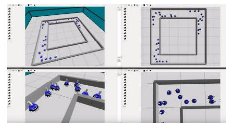
(o) TensorSwarm
