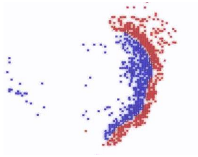
(k) MAgent
